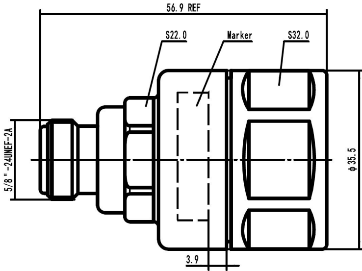
NF-LCF78-C03 Outline drawing
