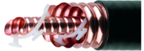
5" Air Dielectric Cable® Air Dielectric Coaxial Cable
