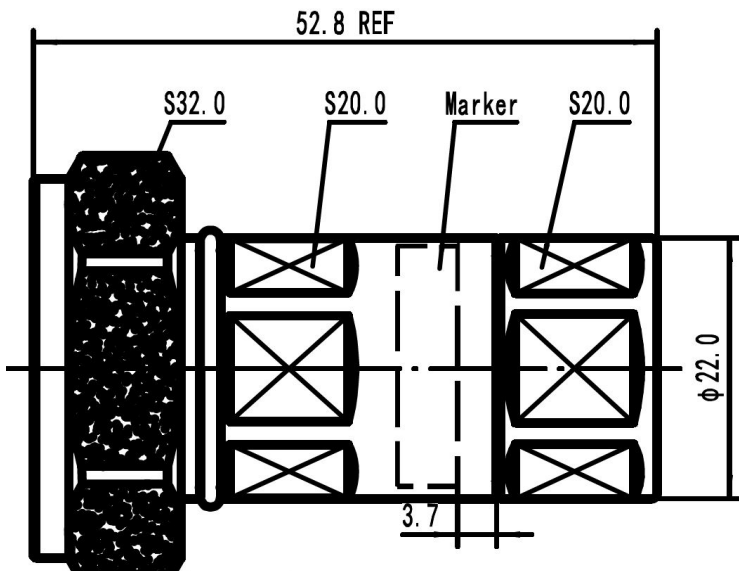
716M-LCF12-C03 Outline drawing
